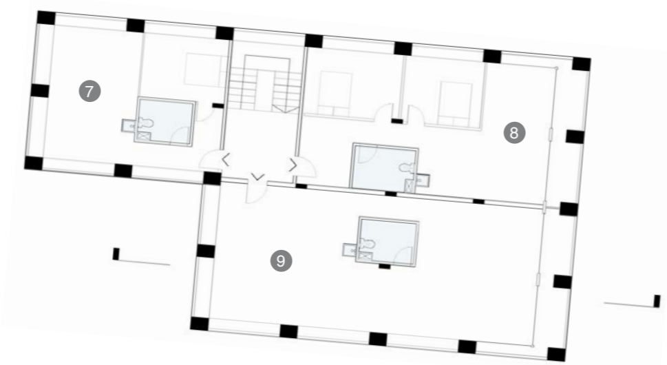
First / Typical Floor Plan: Naked Layout with WC Partition Only Potential Fit Out Options Ghosted.
